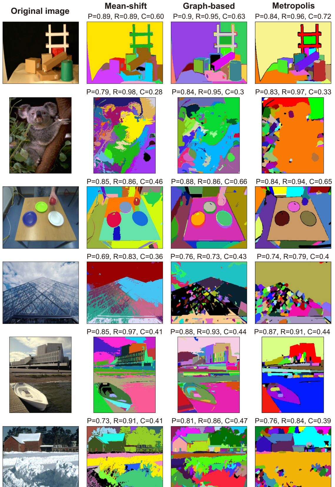
Figure 2.20: Segmentation results on the employed image database (part IV).
