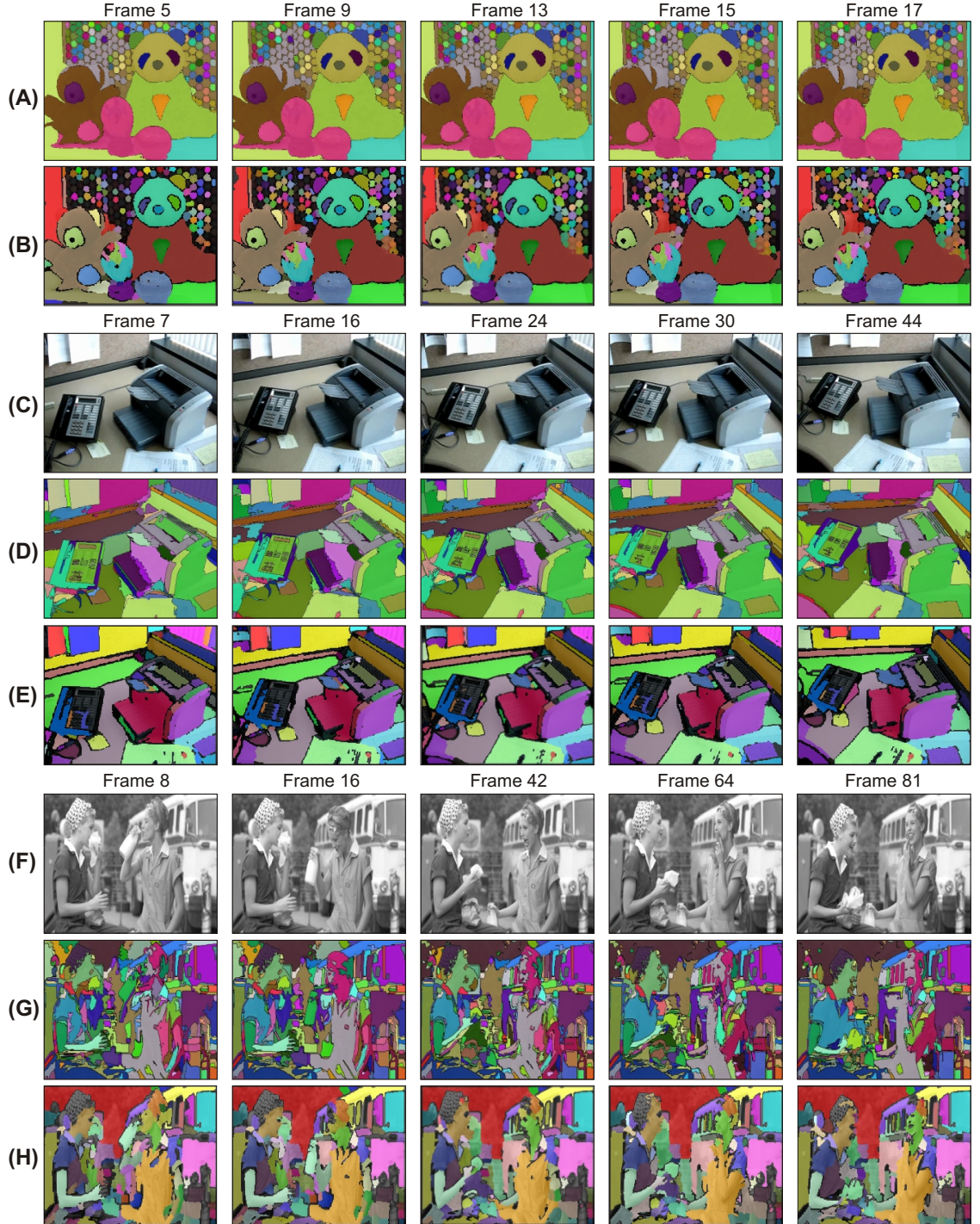
Figure 3.5: Segmentation results for monocular video sequences “Toy” (see Fig. 3.4(A)) and “Phone” (C) with a moving camera and “Women” (F) with moving objects. (A,D,G) Graph-based video segmentation results obtained at 70% (A,D) and 50% (G) of highest hierarchy level. (B,E,H) Segmentation results from the proposed method derived after n_2 = 30 iterations with \alpha_2 = 1.5 (B,E) and \alpha_2 = 2.0 (H), respectively.
