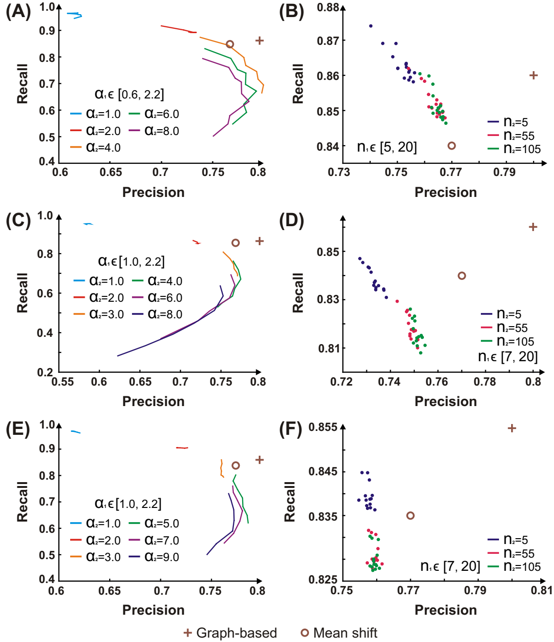
Figure 2.15: Tuning curves for the proposed image segmentation algorithm shown for CIE ( L^*a^*b^* ) (A,B), HSV (C,D), and RGB (E,F) color spaces. The left column shows Precision / Recall scores obtained by changing factor values \alpha_1 and \alpha_2 while holding n_1 and n_2 fixed. The right column, on the contrary, shows Precision / Recall scores obtained by changing iteration numbers n_1 and n_2 holding \alpha_1 and \alpha_2 fixed. Scores for the graph-based and mean shift segmentations are shown as well.
