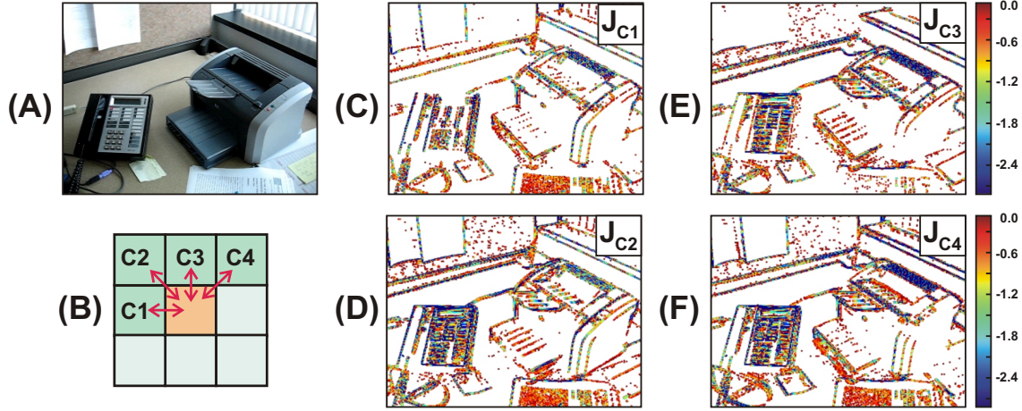
Figure 2.1: Coupling constants for the 8-connectivity case in the CIE ( L^*a^*b^* ) color space. (A) Original image. (B) Mask for eight-connected connectivity. (C - F) Matrices with coupling constants computed for horizontal, left diagonal, vertical and right diagonal directions. Note that only coupling constants leading to the formation of segments are shown here ( J < 0 ).
