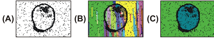
Figure 2.12: Fast connected-component labeling. (A) Computed region boundaries. (B) Provisional labels assigned after the first image scan. (C) Representative labels assigned after the second image scan.
