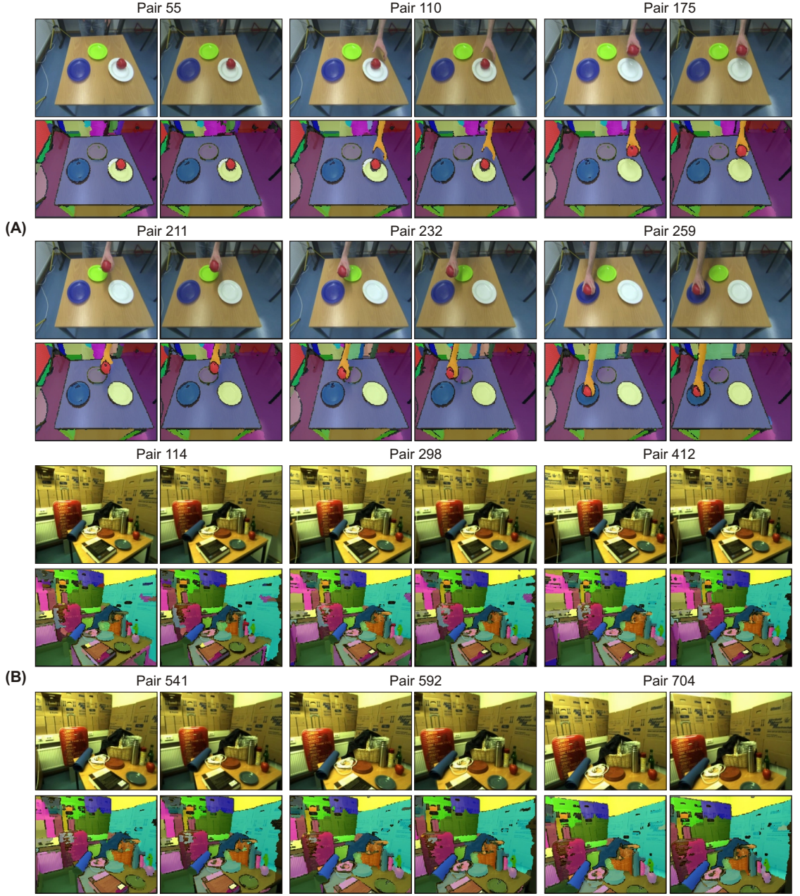
Figure 4.3: Segmentation results for stereo frame sequences of the sample actions “Moving an apple over plates” with moving objects (A) and “Cluttered scene” with a moving stereo camera (B). Results are obtained using the following parameters: n_2 = 30 and n_2 = 15 iterations are applied for the relaxation of left and right frames, respectively, \alpha_2 = 2.5 for both the left and right streams, the annealing schedule is T_{n+1} = 0.999 \cdot T_n starting with T_0 = 1.0 .
